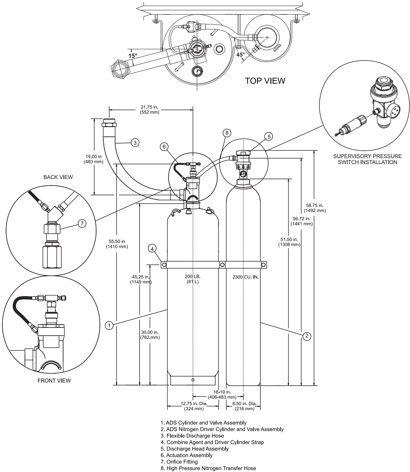
Figure 1. Nitrogen and Agent Cylinders
